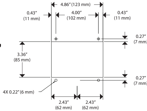
Three (3) Sensor Top View
