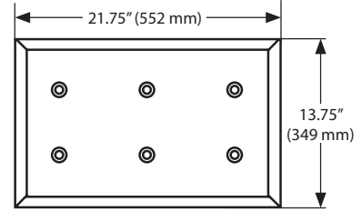
Six (6) Sensor Top View
